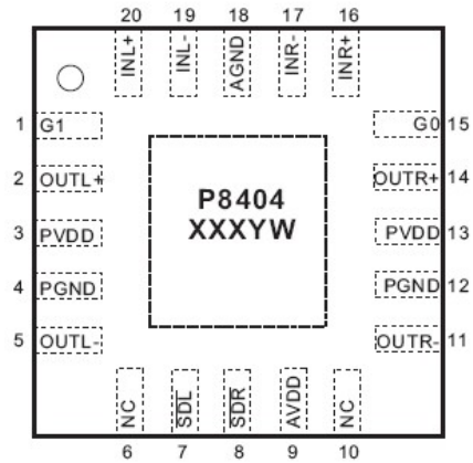
QFN 4mmx4mm Top View
