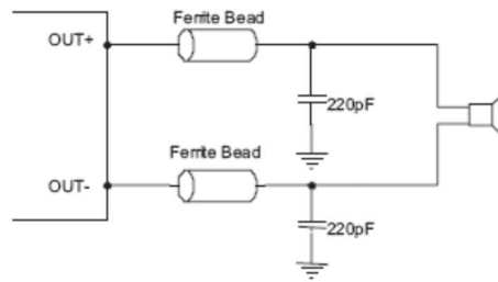
Figure 1. Ferrite Bead Filter to Reduce EMI
