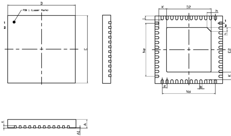
QFN 48L (0606X0.75-0.40) (B)
